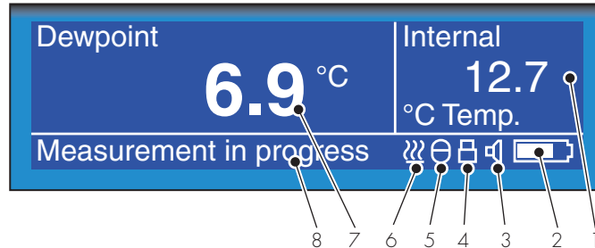
Figure 3 Instrument Display
