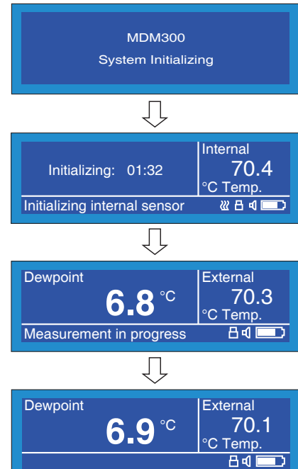
Figure 15 Start-Up Sequence
