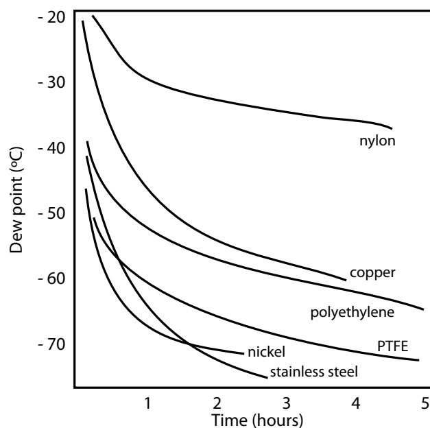
Figure 4 Material Permeability Comparison
